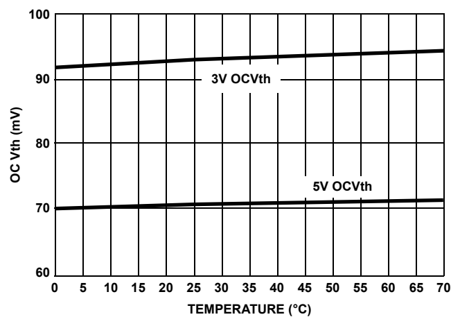
FIGURE 4. OCVth vs TEMPERATURE ( V_{ROSET} = 1.21V )
