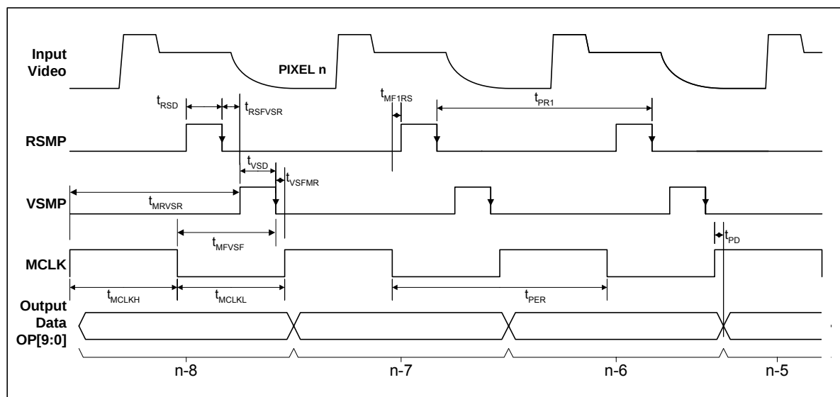
Figure 2 One-channel CDS Operation (CDS=1)
