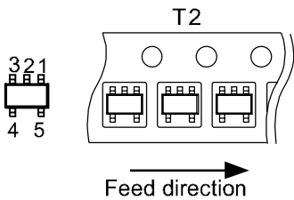
No. : MP005-A-C-SD-1.0
