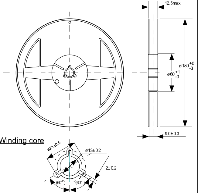
No. MP005-A-R-SD-1.0
