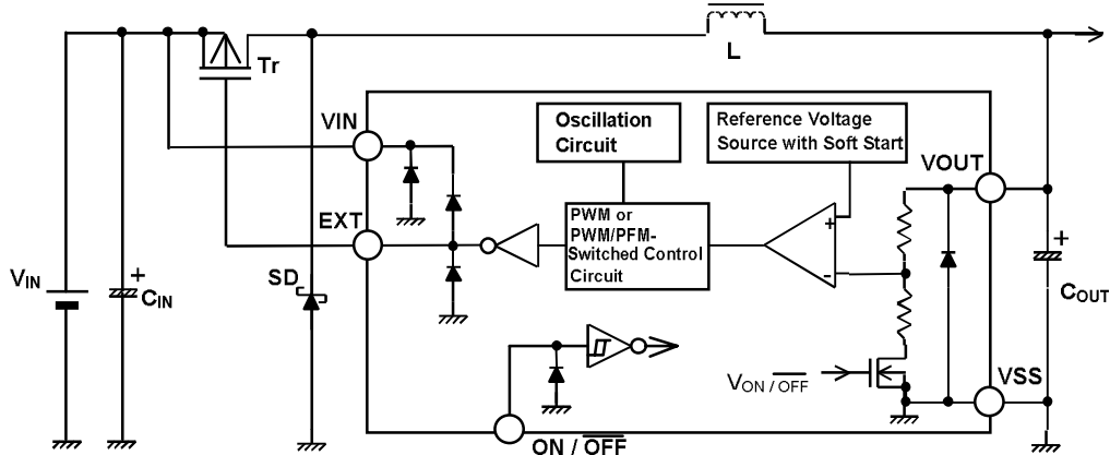
Figure 1 Block Diagram
