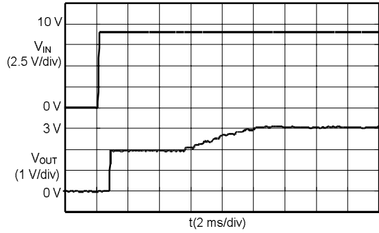
S-8520/1C30MC ( V_{IN} :0 →9.0 V)
