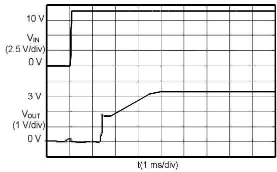
S-8520/1E33MC ( V_{IN} :0 →9.0 V)
