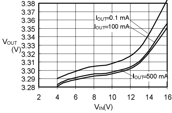
V_{OUT}-V_{IN} S-8521F33MC (Ta=25°C)
