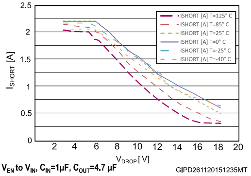
Figure 25: Short-circuit current vs dropout voltage ( V_{OUT} = V_{ADJ} )
