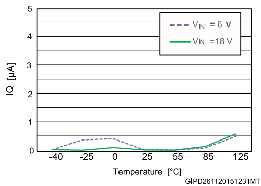
Figure 22: Off-state current vs temperature ( V_{OUT} = 5\text{ V} )
