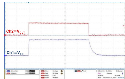
Figure 33: Startup with enable ( V_{OUT} = V_{ADJ} )
