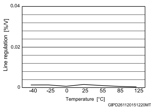
Figure 10: Line regulation vs temperature ( V_{IN} = 6\text{ to }18\text{ V} , V_{OUT} = 5\text{ V} , I_{OUT} = 10\text{ mA} )
