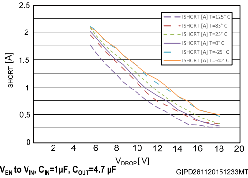
Figure 24: Short-circuit current vs dropout voltage ( V_{OUT} = 5\text{ V} )
