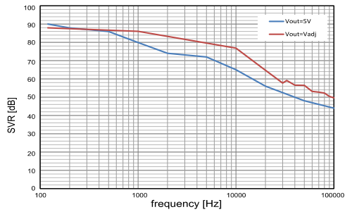
Figure 26: SVR versus frequency
