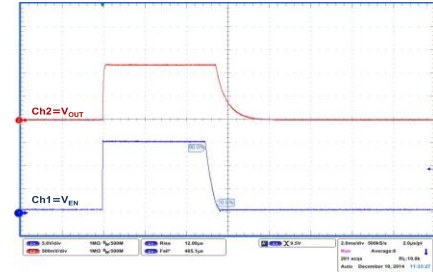
Figure 35: Turn-on time ( V_{OUT} = V_{ADJ} )
