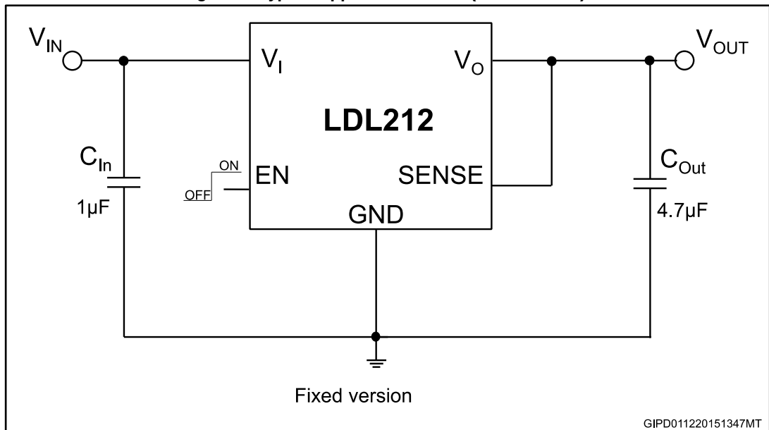
Figure 5: Typical application circuit (fixed version)
