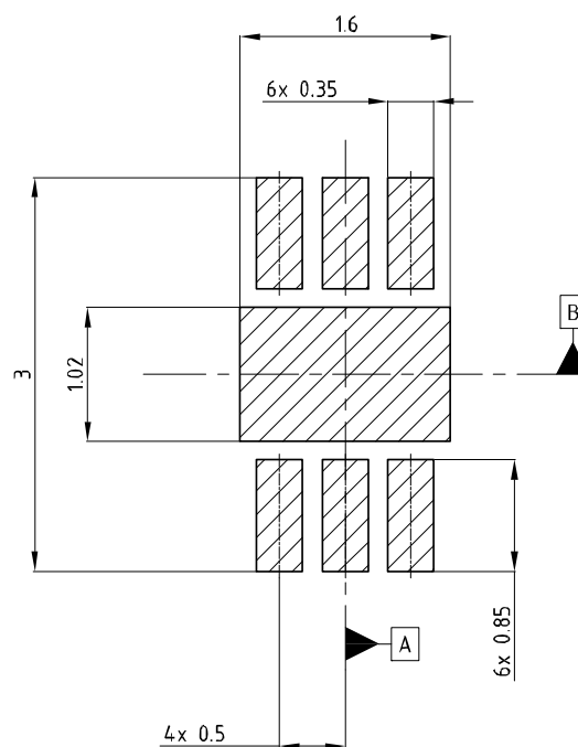
Figure 45: DFN6 (2x2) recommended footprint
