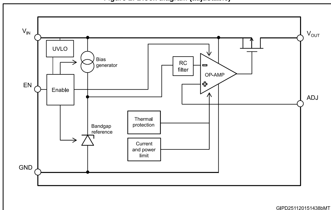
Figure 2: Block diagram (adjustable)
