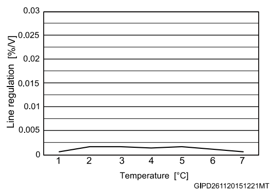
Figure 11: Line regulation vs temperature ( V_{IN} = 2.5\text{ to }18\text{ V} , V_{OUT} = V_{ADJ} , I_{OUT} = 10\text{ mA} )
