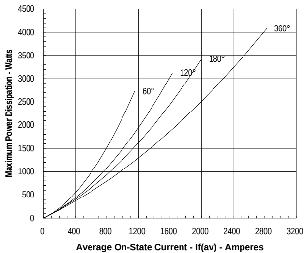
Maximum On-State Power Dissipation
