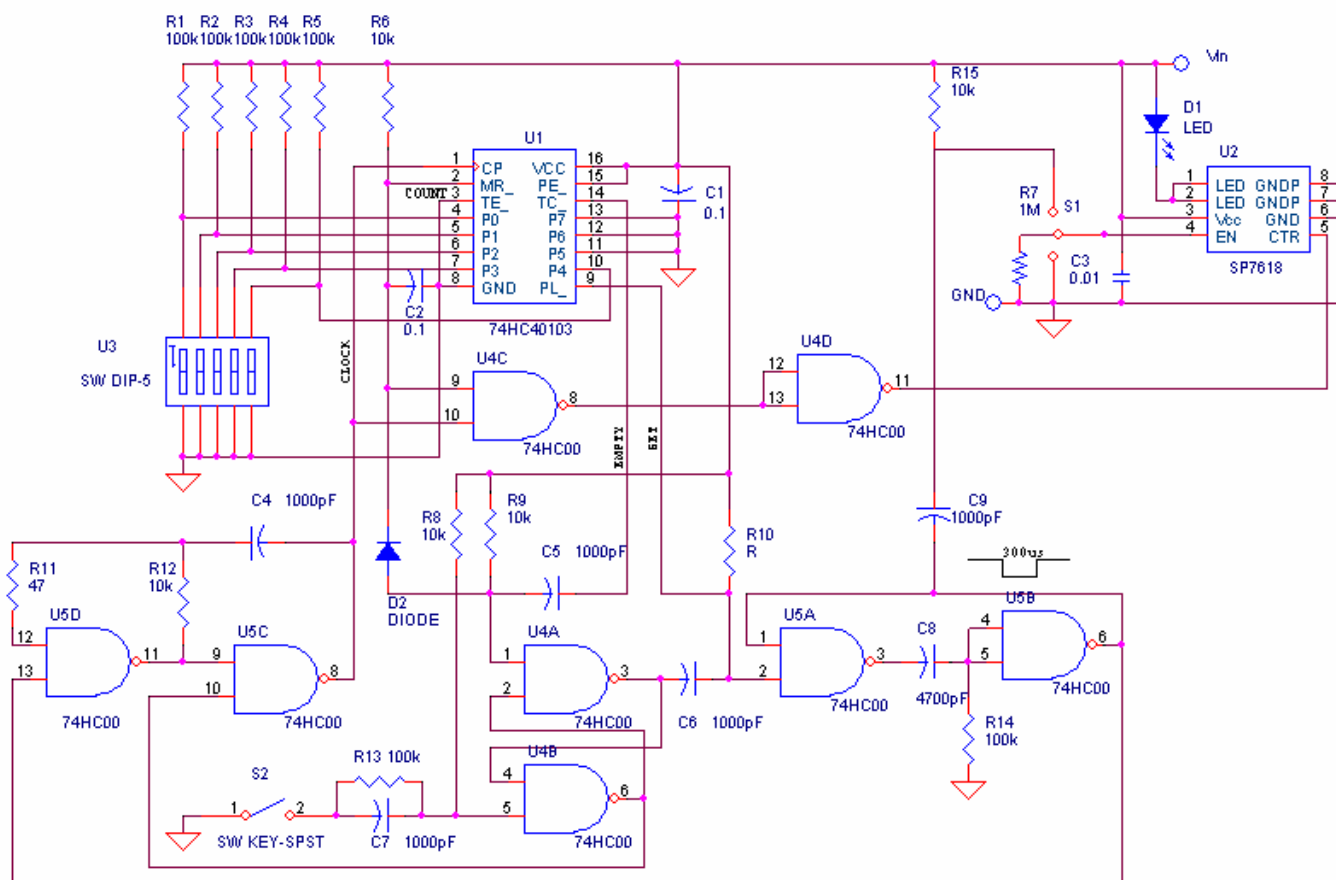
Figure 1. SP7618 Evaluation Board Schematic Diagram
