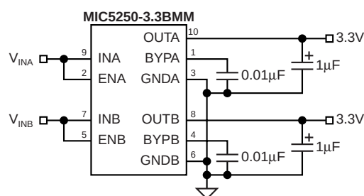
Figure 1. Ultra-Low-Noise Dual 3.3V Application
