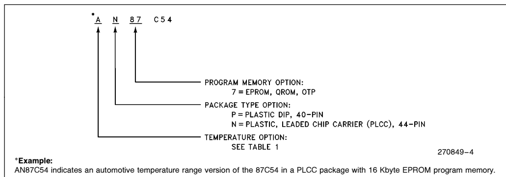
Figure 2. Package Options
