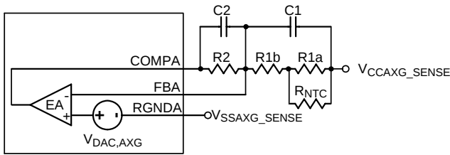
Figure 20. AXG VR : Loop Setting with Temperature Compensation
