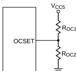
Figure 17. OCP Setting without Temperature Compensation
