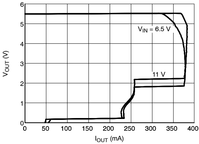
Figure 5. Output Voltage vs. Output Current 5.5 V Version ( T_J = 25^\circ\text{C} )
