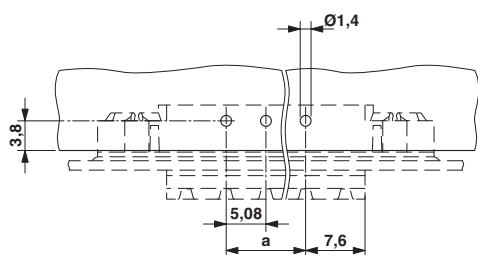
Drilling diagram
