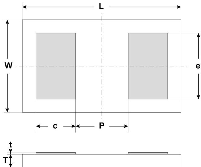
Figure 6 – Layout view
