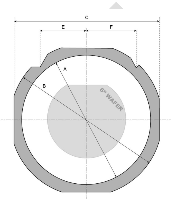
Figure 13 FF108 Frame with a 6 inch wafer
