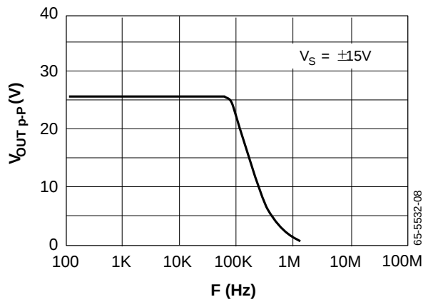
Figure 5. Output Voltage Swing vs. Frequency
