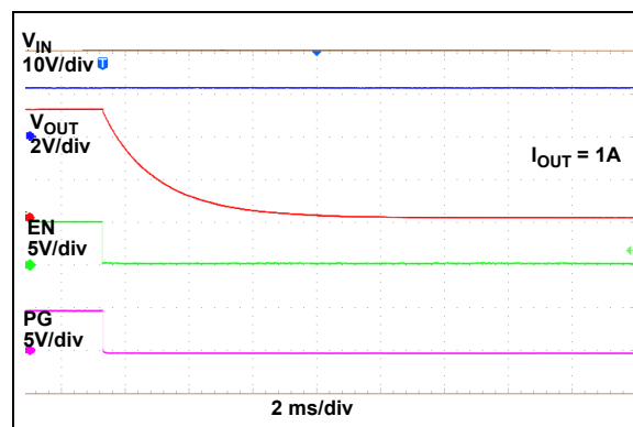
FIGURE 2-29: Enable Turn-Off.
