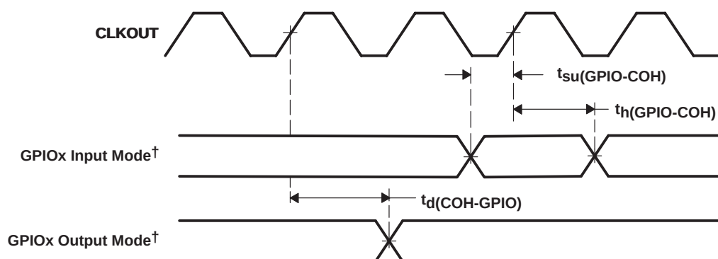
Figure 5-31. GPIOx ^\dagger Timings
