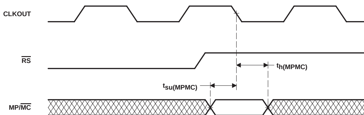
Figure 5-17. \text{MP}/\overline{\text{MC}} Timing
