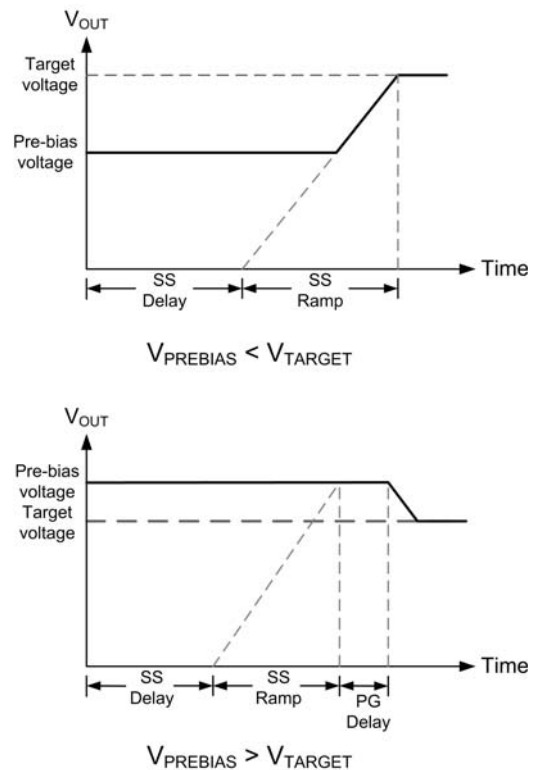
FIGURE 15. OUTPUT RESPONSES TO PREBIAS VOLTAGES
