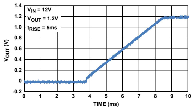
FIGURE 9. SOFT-START RAMP-UP
