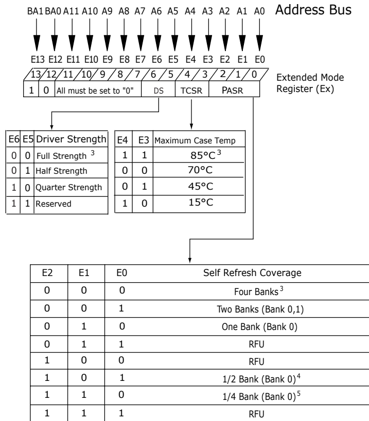
Figure 33.I Extended Mode Register
