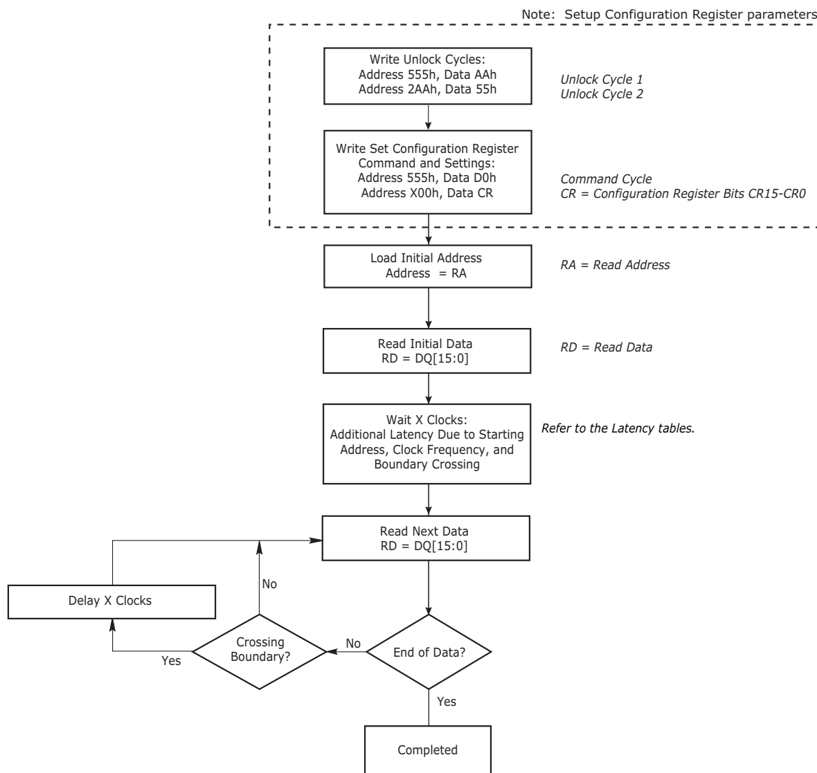
Figure 12.2. Synchronous Read
