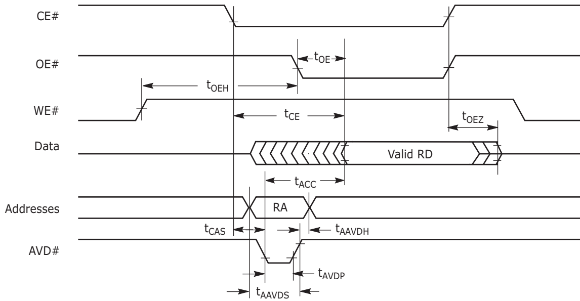
Figure I6.II. Asynchronous Mode Read
