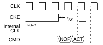
Figure 65.10 Clock Suspend Exit and Power Down Exit
