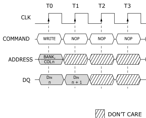
Figure 47.2. Write Burst
