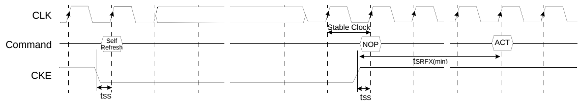
Figure 65.I2 Self Refresh
