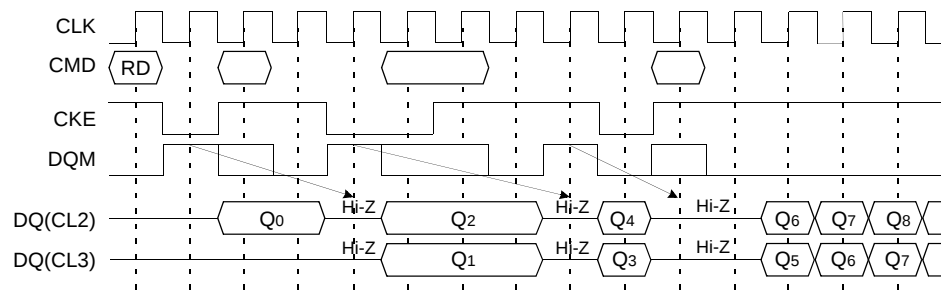
Figure 65.2 DQM Operation
