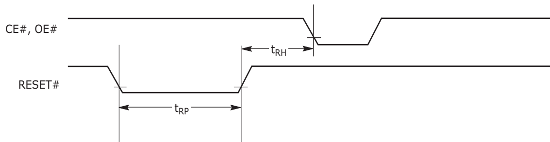
Figure 16.13. Reset Timings
