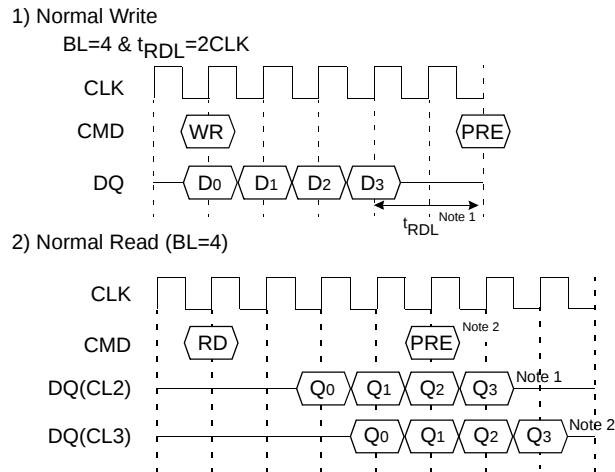
Figure 65.6 Precharge
