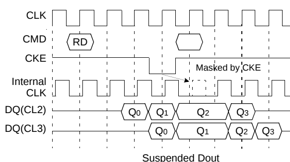
Figure 65.1 Clock Suspend
