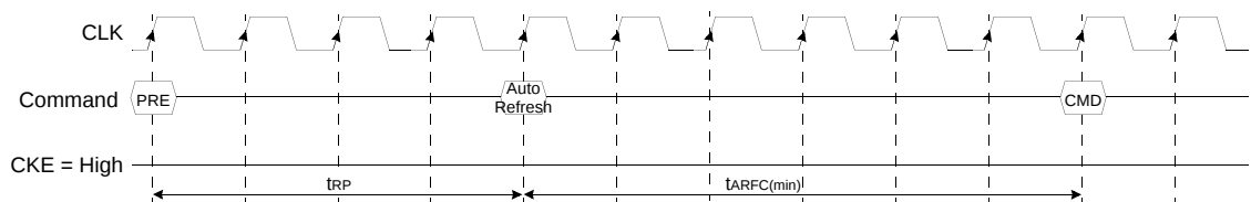
Figure 65.11 Auto Refresh
