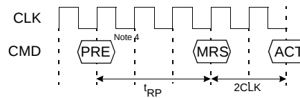
Figure 65.9 MRS
