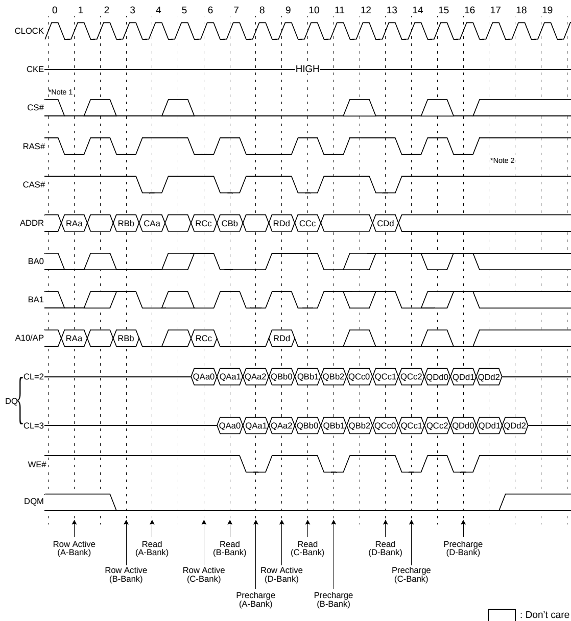
Figure 70.5 Page Read Cycle at Different Bank @Burst Length=4
