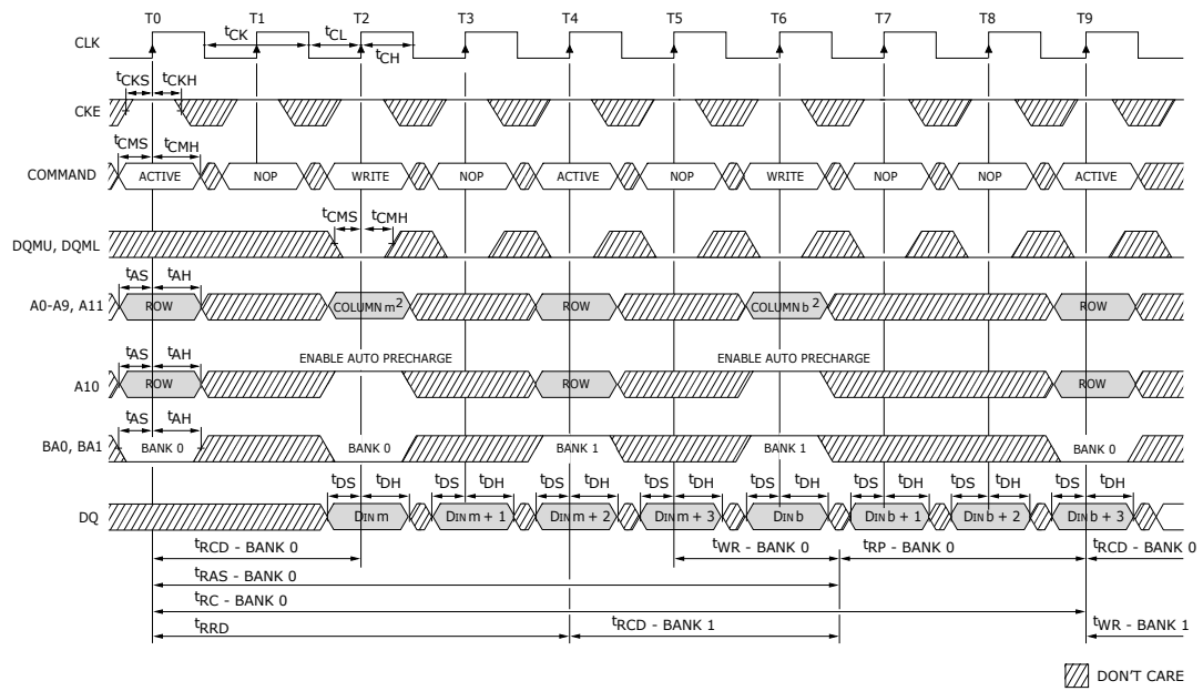
Figure 48.I7. Alternating Bank Write Accesses
