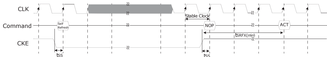
Figure 87.15 Self Refresh
