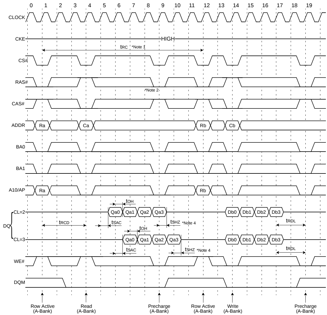
Figure 70.3 Read & Write Cycle at Same Bank @Burst Length=4, t_{RDL}=2CLK
