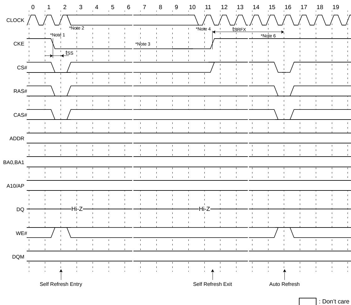
Figure 70.15 Self Refresh Entry & Exit Cycle
