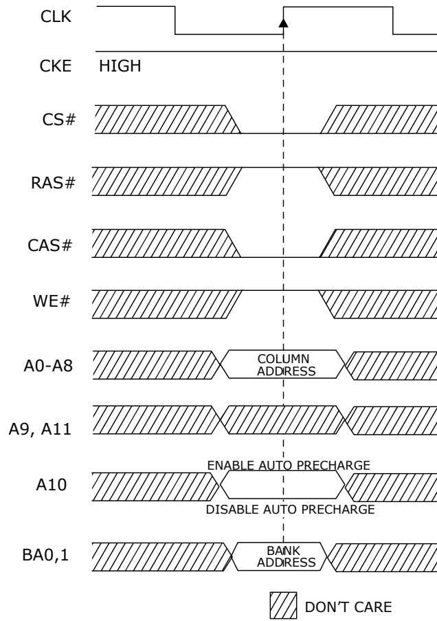
Figure 47.1 Read Command
