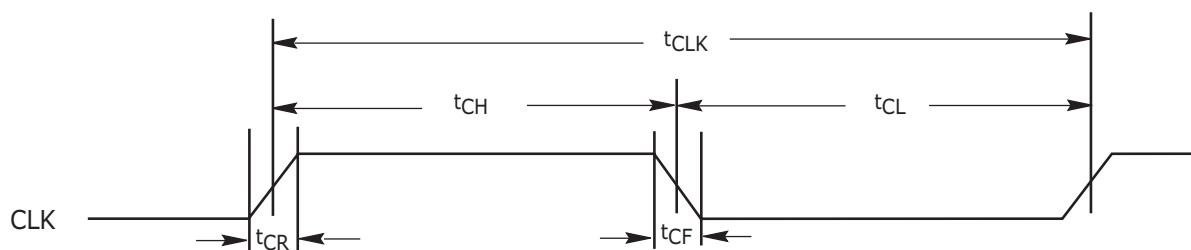
Figure 16.6. CLK Characterization
