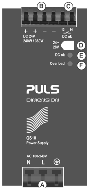
Fig. 13-1 Front side
