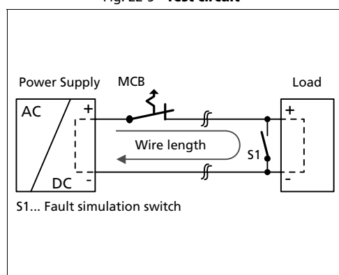
Fig. 22-5 Test circuit
