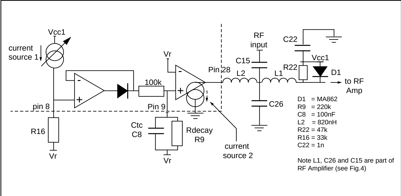
Fig.6 AGC Schematic
