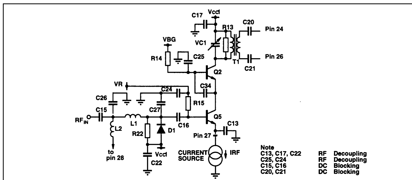
Fig.4 RF amplifier
