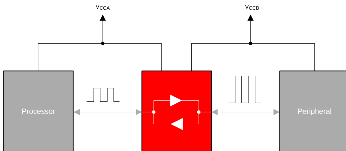
Typical Application Block Diagram for TXB010X
