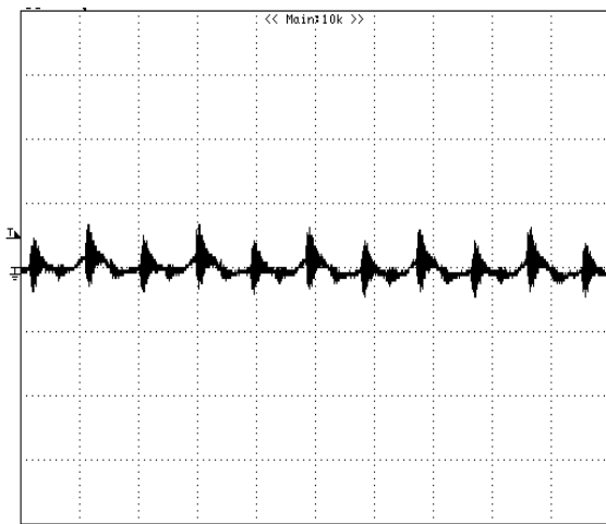
Figure 14: Output voltage ripple at nominal input voltage and rated load current ( I_o=40\text{A} ) (20 mV/div, 2 \mu\text{s} /div) Load capacitance: 1\mu\text{F} ceramic capacitor and 10\mu\text{F} tantalum capacitor. Bandwidth: 20 MHz. Scope measurements should be made using a BNC cable (length shorter than 20 inches). Position the load between 51 mm to 76 mm (2 inches to 3 inches) from the module.
