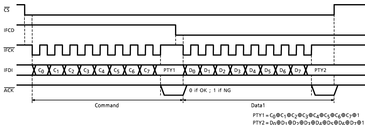
Fig.10 (b) Example of Timing for 9bit Transfer Mode
