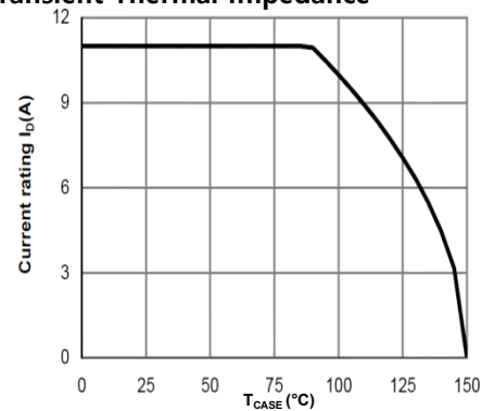
Figure 15: Current De-rating
