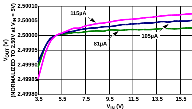
FIGURE 4. LINE REGULATION
