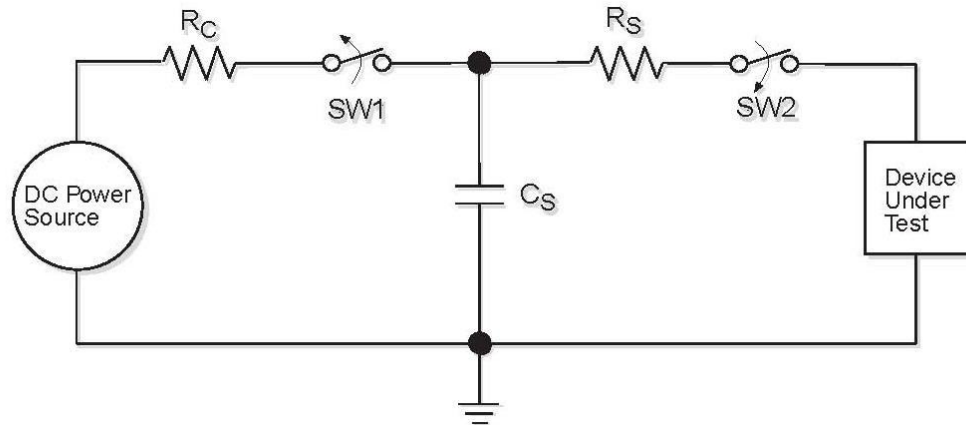
Fig. 1 ESD Test Circuit for Human Body Model
