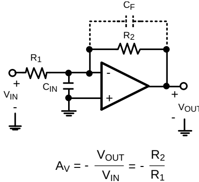
Figure 46. Compensating for Input Capacitance
