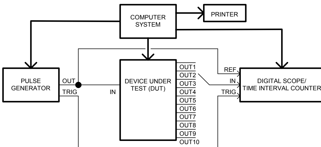
Figure 2: Test Setup
