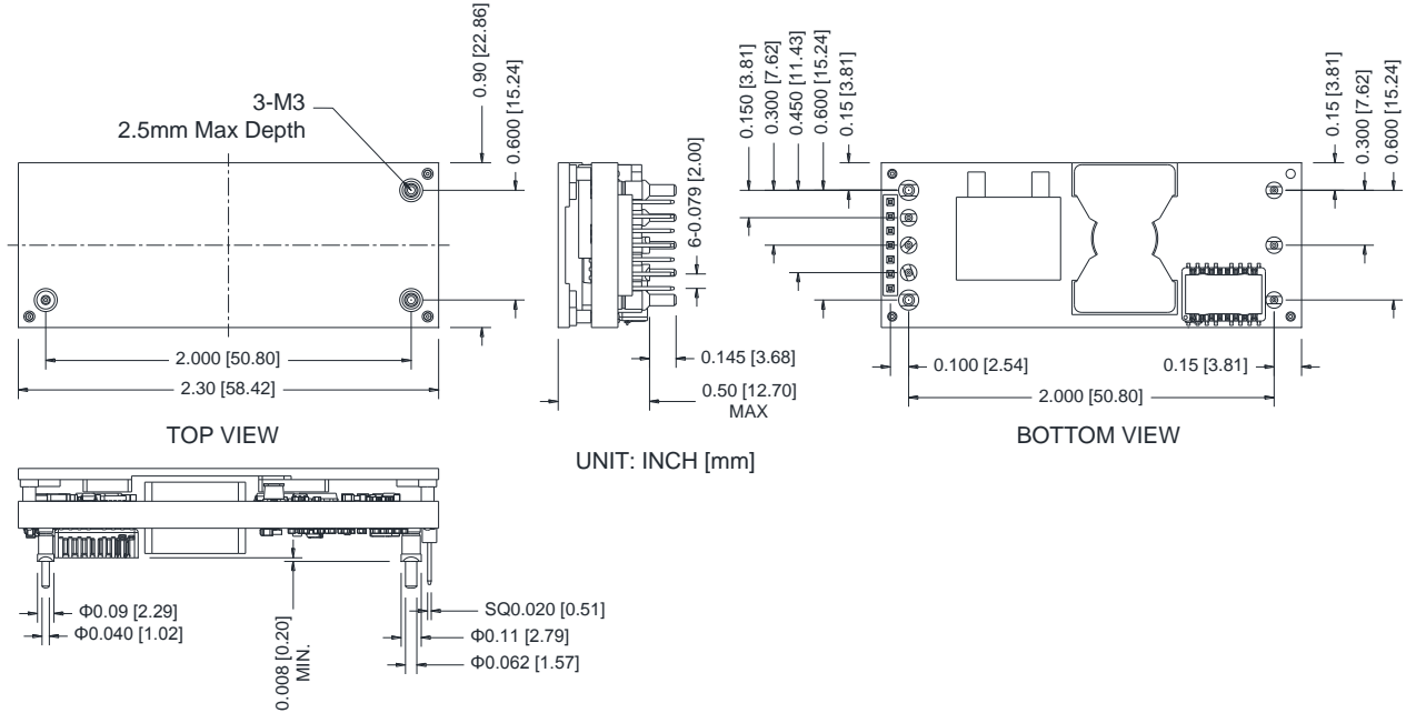
Figure 37. 0RCP-D4T12A/0RCP-D4T12B outline
