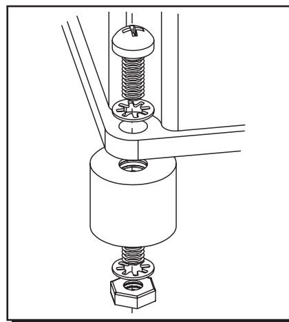
Figure 1 Mounting the Points Box.
