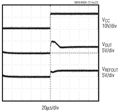
STARTUP DELAY
