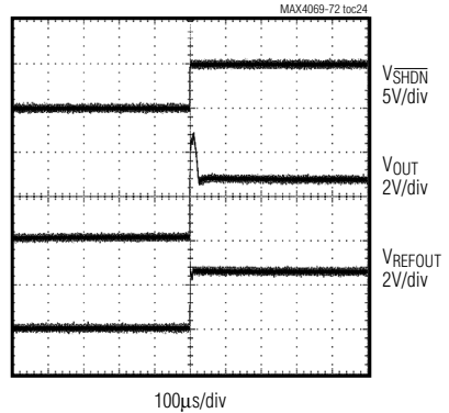
EXITING SHUTDOWN
