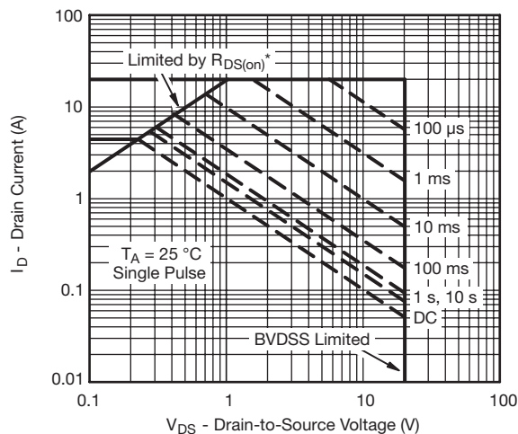
* V_{GS} > \text{minimum } V_{GS} \text{ at which } R_{DS(on)} is specified Safe Operating Area, Junction-to-Ambient
