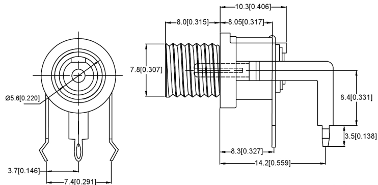
MATING PLUG Jack Insertion Depth: 9.0 mm
