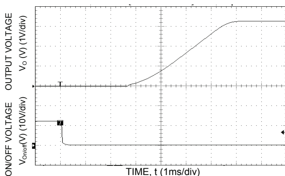
Figure 15. Typical Start-Up Using Remote On/Off with Low-ESR external capacitors (7x150μF Polymer) ( V_{IN} = 12.0\text{Vdc} , V_o = 3.3\text{Vdc} , I_o = 3\text{A} , C_o = 1050\mu\text{F} ).
