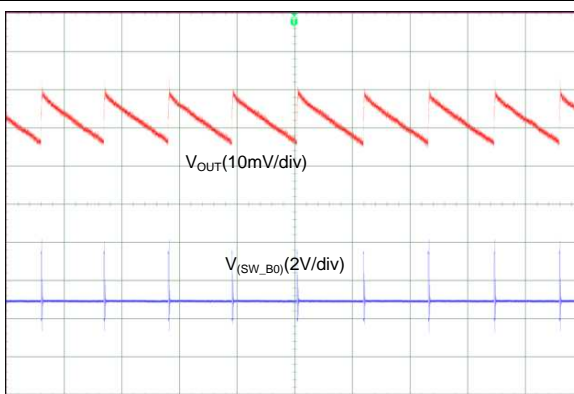
Figure 78. Output Voltage Ripple, PFM Mode (3-Phase Output)
