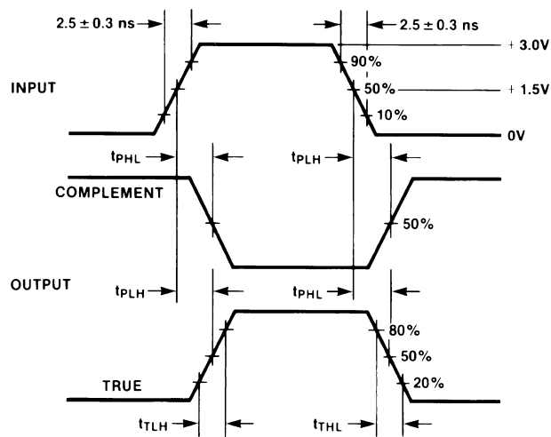
Figure 3. Propagation Delay and Transition Times
