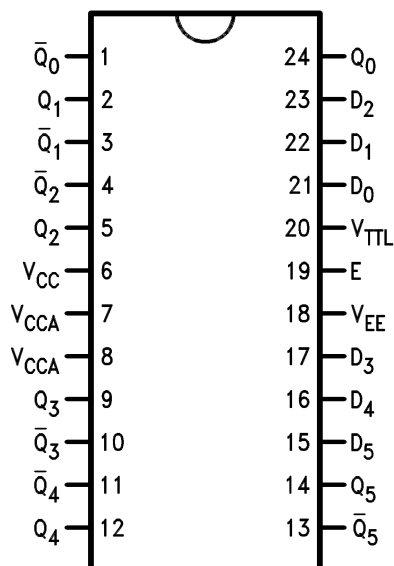
Figure 1. 24-Pin CDIP
