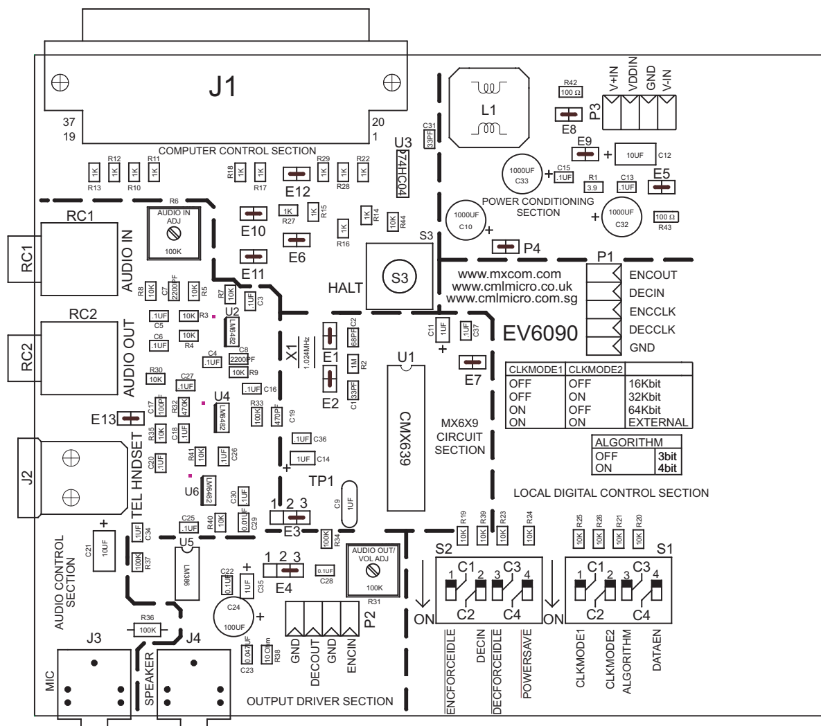
Figure 8: Evaluation Board Layout
