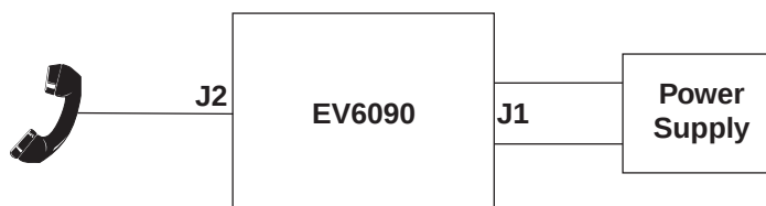
Figure 4: POTS Set-Up
