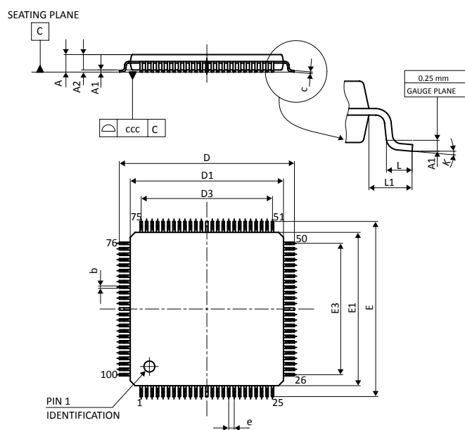
Figure 85. LQFP100 - Outline
