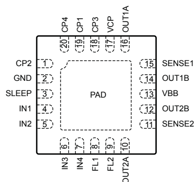
Pin-out Diagram
