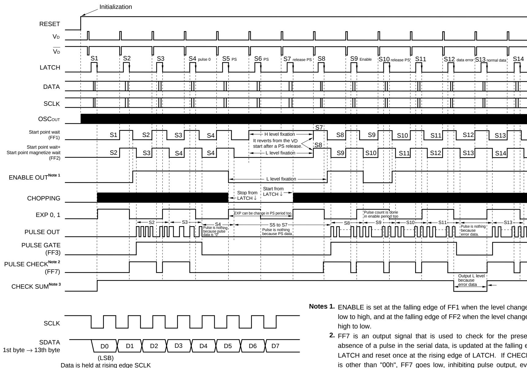
TIMING CHART (1)
