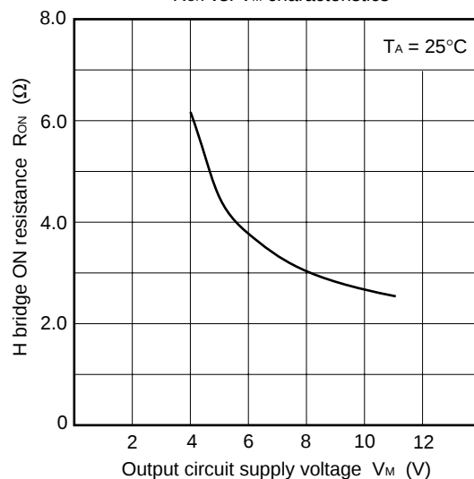
R_{\text{ON}} vs. V_M characteristics
