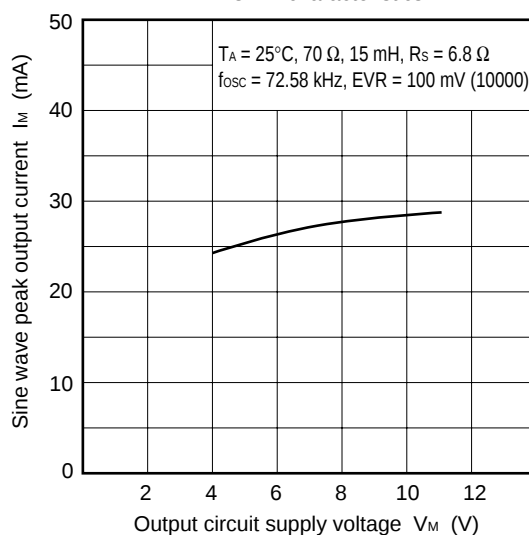
I_M vs. V_M characteristics
