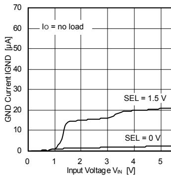
Fig. 4 GND Current vs Input Voltage (BH12PB1WHFV)
