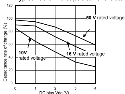
Fig. 28 Capacitance vs Bias (Y5V)
