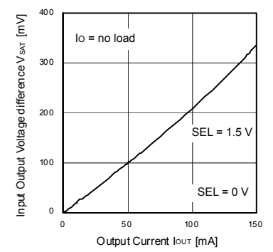
Fig. 6 Input Output Voltage difference vs Output Current (BH33PB1WHFV)
