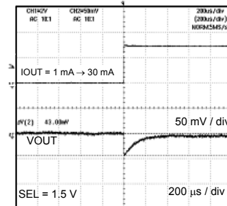
Fig. 20 Load Response ( C_O = 1.0 \mu F ) (BH30PB1WHFV)
