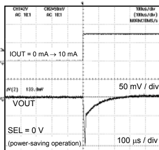
Fig. 19 Load Response ( C_O = 1.0 \mu F ) (BH30PB1WHFV)
