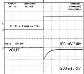
Fig. 21 Load Response ( C_O = 1.0 \mu F ) (BH30PB1WHFV)
