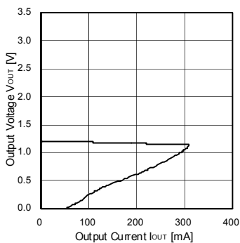
Fig. 10 Dropout voltage vs Output Current (BH12PB1WHFV)
