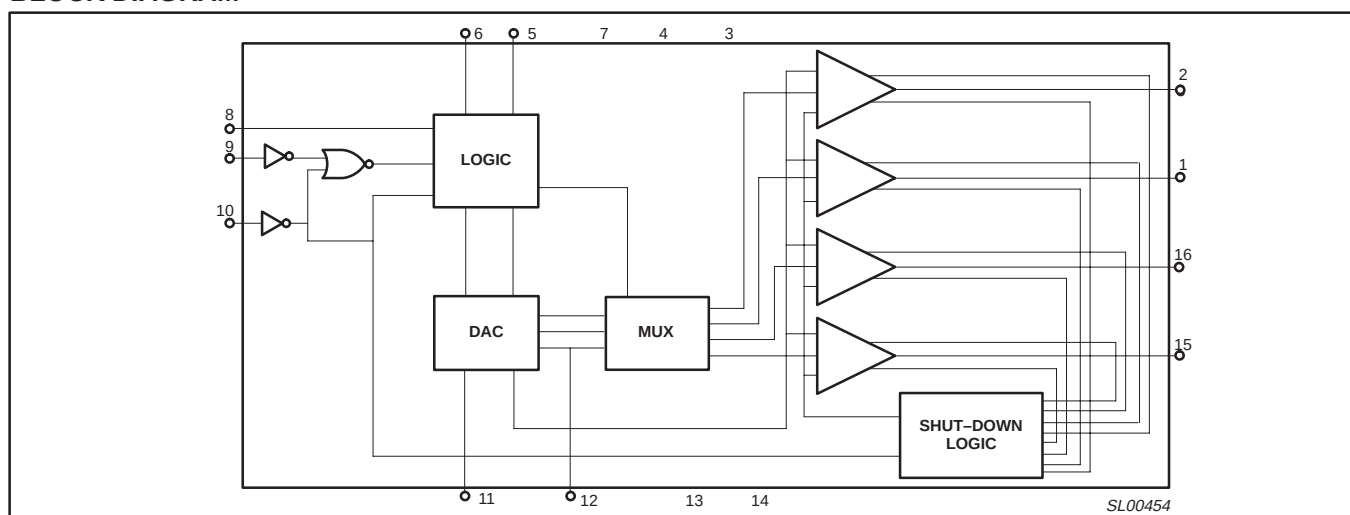
Figure 2. Block diagram
