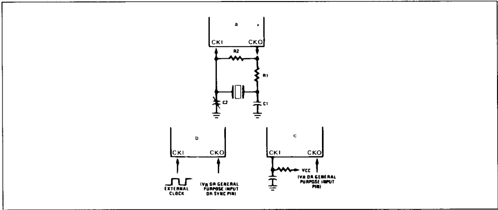
Figure 4 : ETL9420/L9421/L9422 Oscillator.
