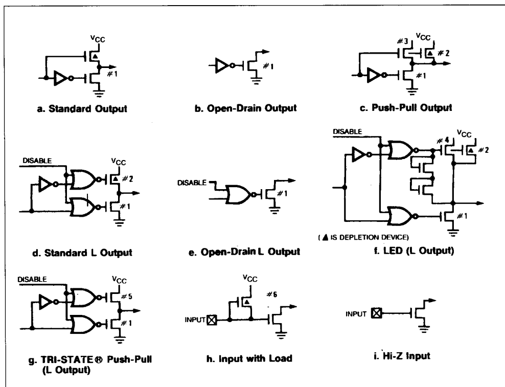
Figure 5 : Output Configurations.
