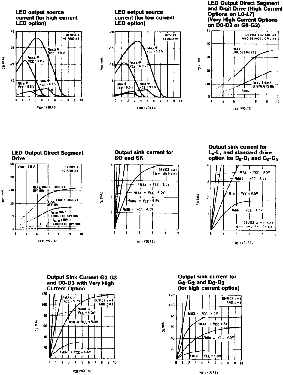
Figure 6 : ETL9420/L9421/L9422 Input/Output Characteristics (continued).
