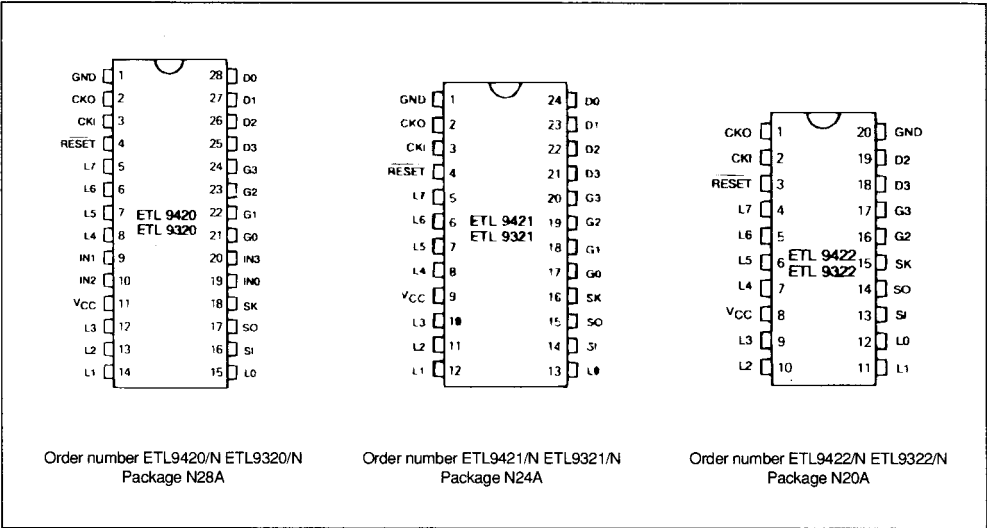
Figure 2 : Connection Diagrams.
