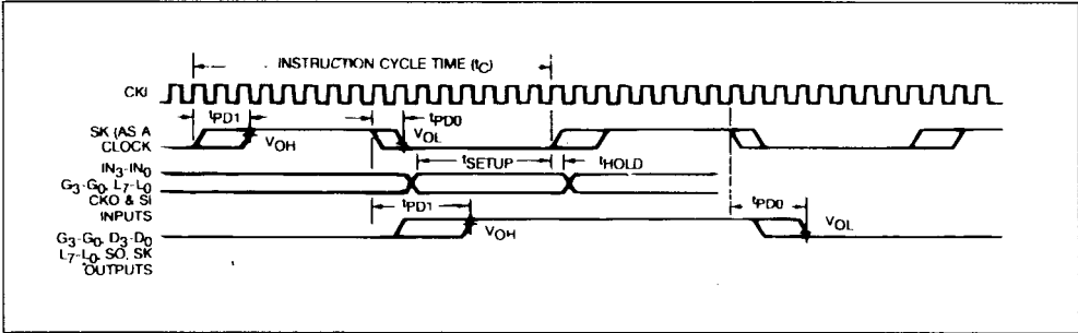
Figure 3 : Input/Output Timing Diagrams (crystal divide-by-16 mode).
