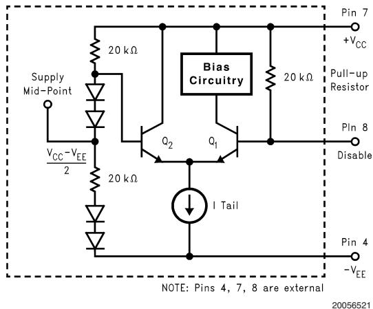
FIGURE 4. Enable/Disable Operation
