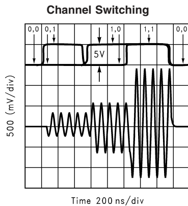
FIGURE 7. PGA Output
