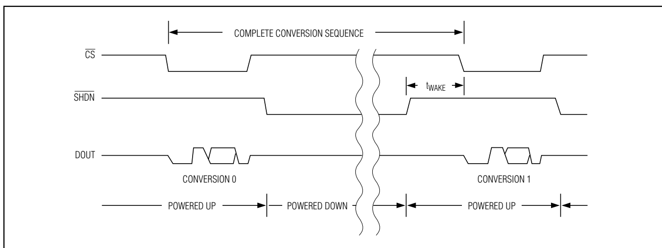
Figure 5. Shutdown Sequence
