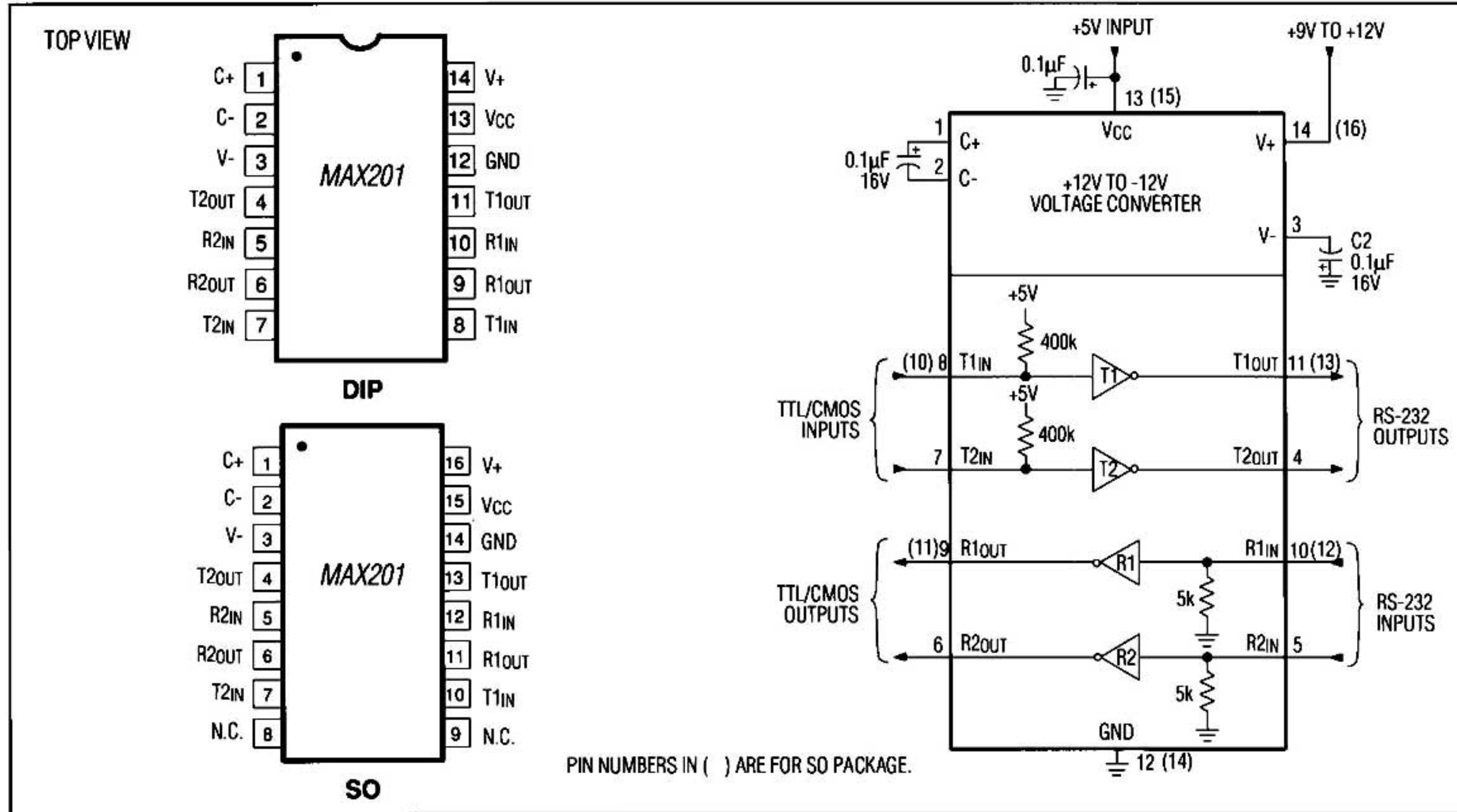
Figure 7. MAX201 Pin Configurations and Typical Operating Circuit
