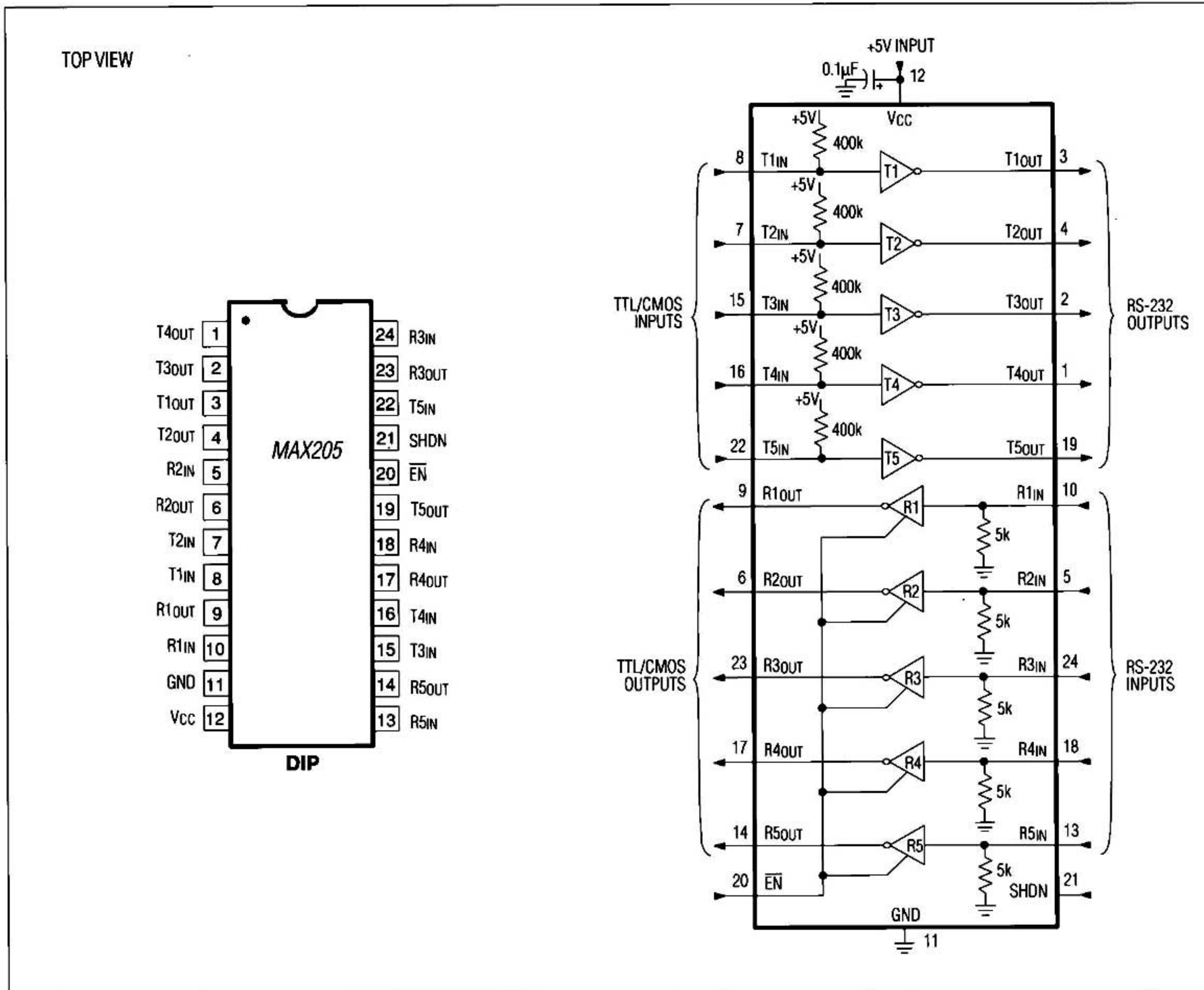
Figure 11. MAX205 Pin Configuration and Typical Operating Circuit
