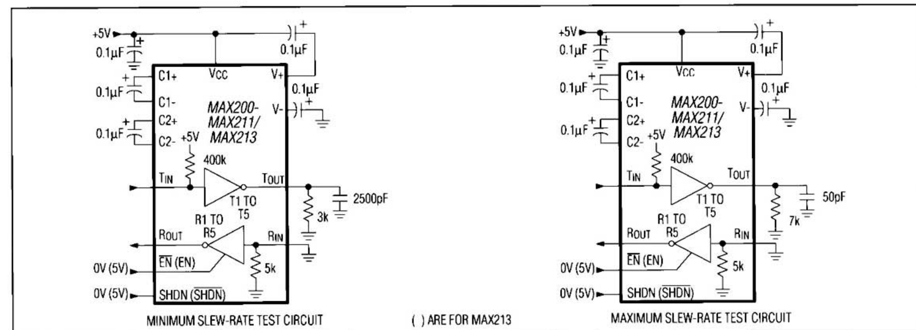
Figure 3. Transition Slew-Rate Test Circuit
