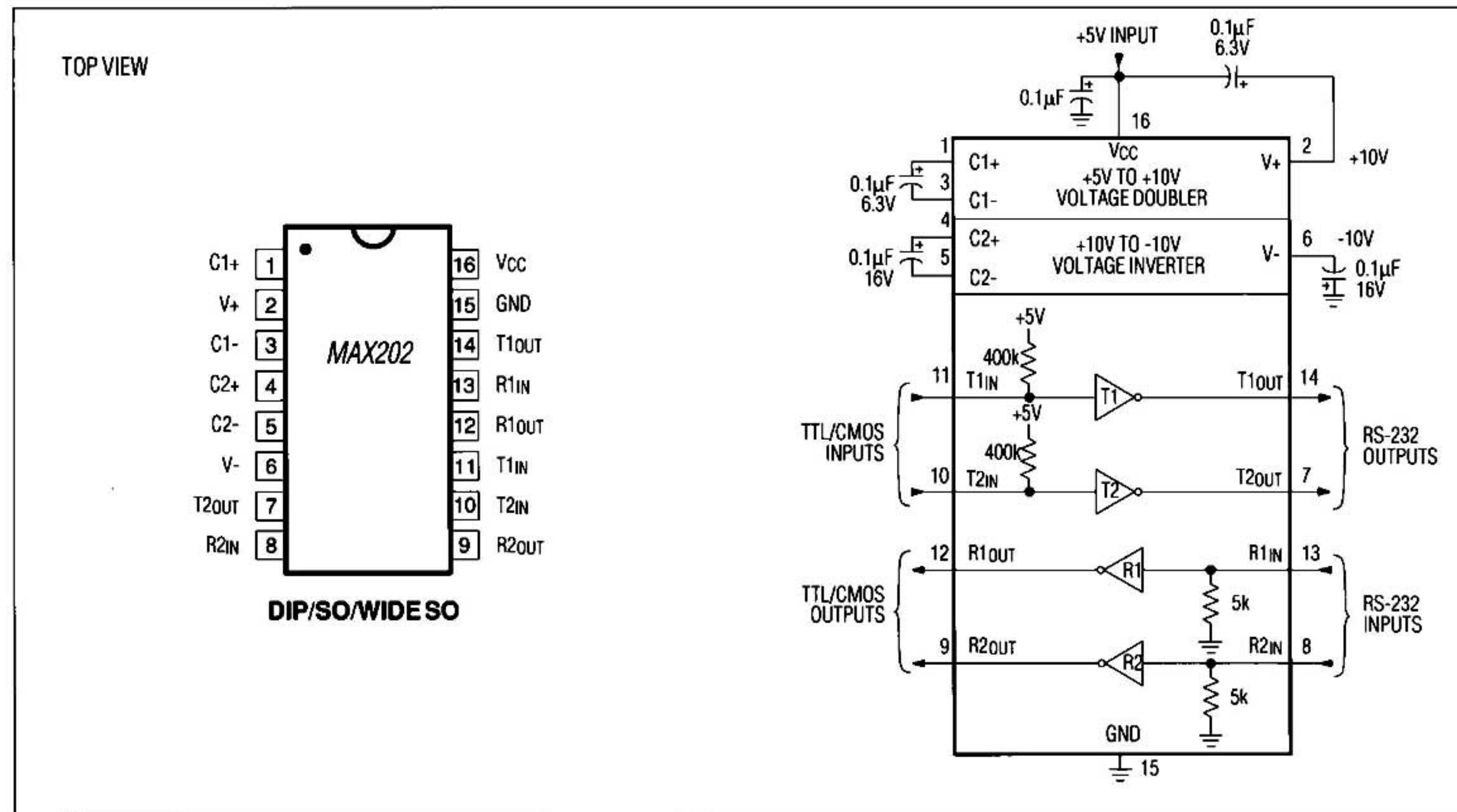
Figure 8. MAX202 Pin Configuration and Typical Operating Circuit
