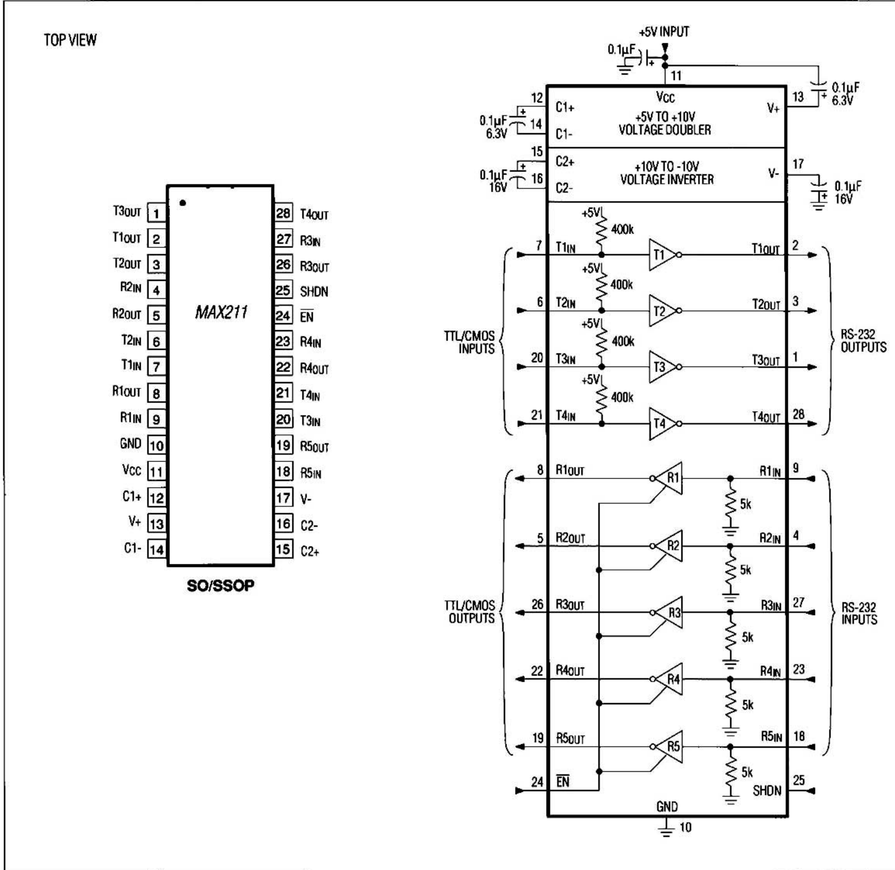
Figure 16. MAX211 Pin Configuration and Typical Operating Circuit
