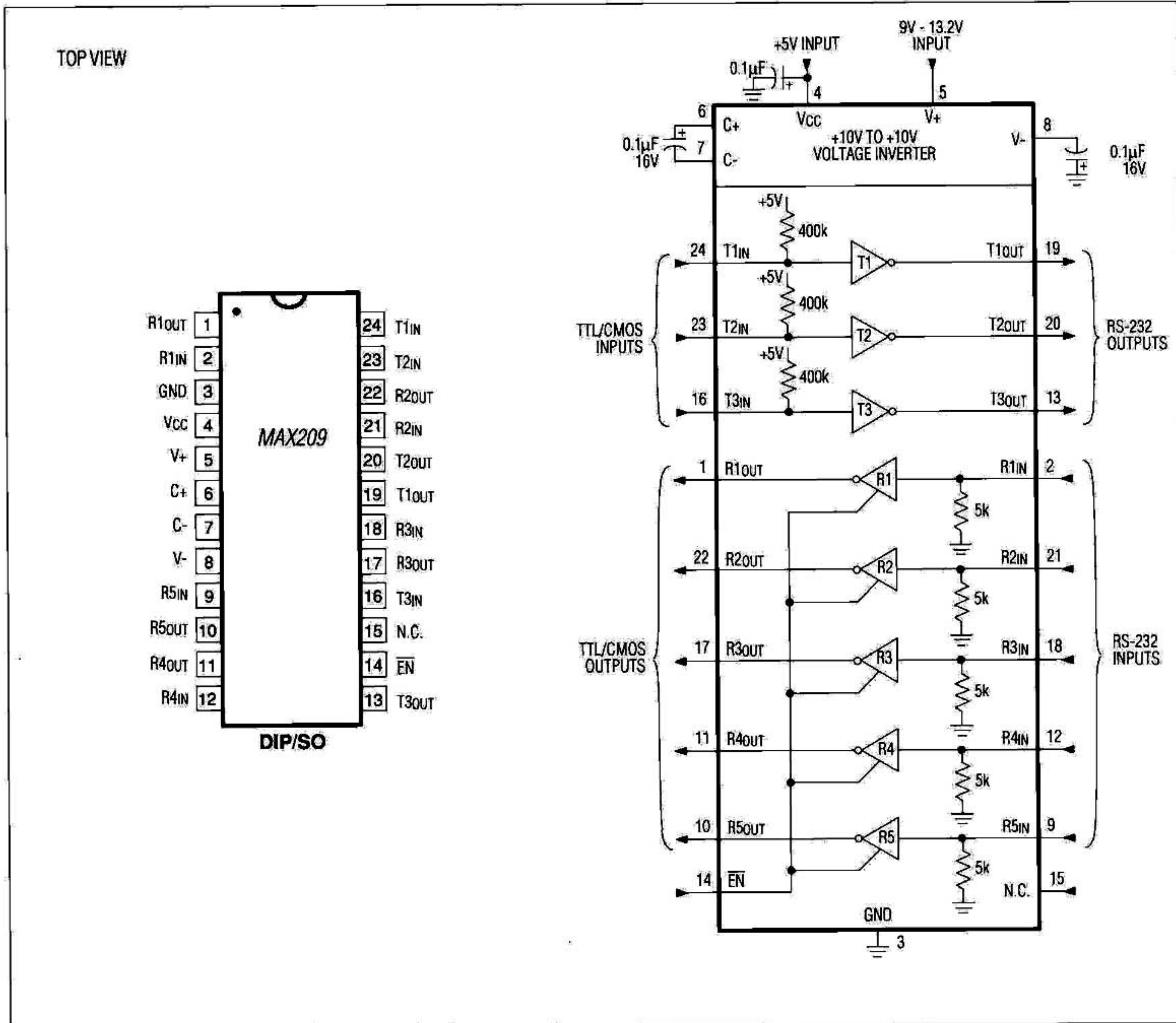
Figure 15. MAX209 Pin Configuration and Typical Operating Circuit
