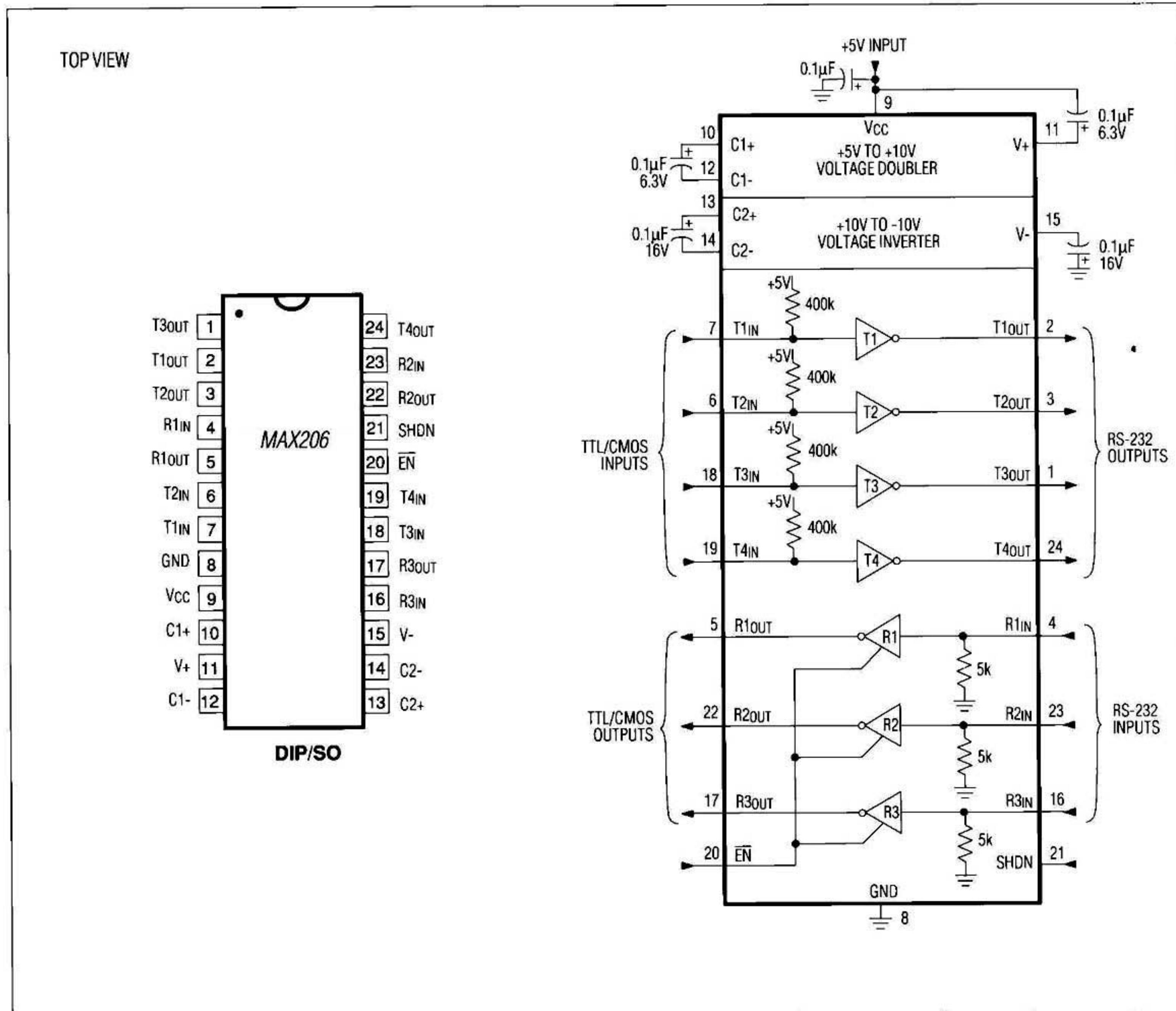
Figure 12. MAX206 Pin Configuration and Typical Operating Circuit
