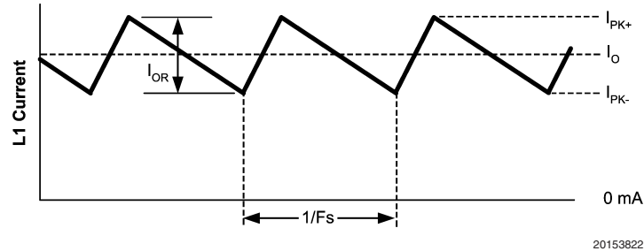
FIGURE 5. Inductor Current
