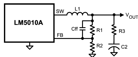
FIGURE 10. Low Output Ripple Using a Feedforward Capacitor
