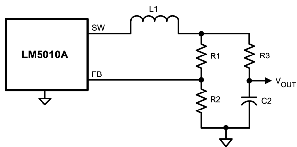
FIGURE 9. Low Ripple Output
