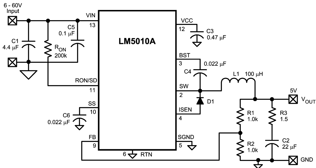
FIGURE 6. Example Circuit
