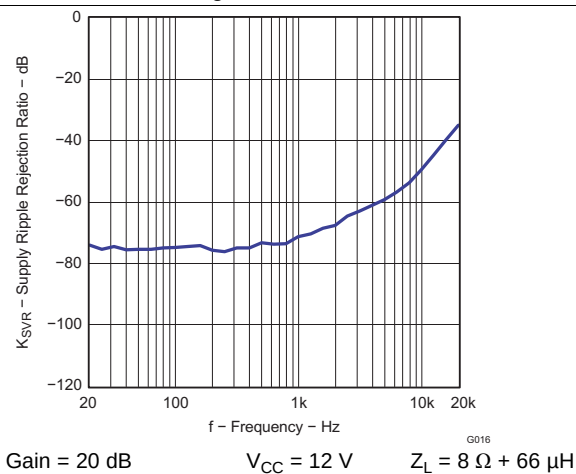
Figure 14. Supply Ripple Rejection Ratio vs Frequency
