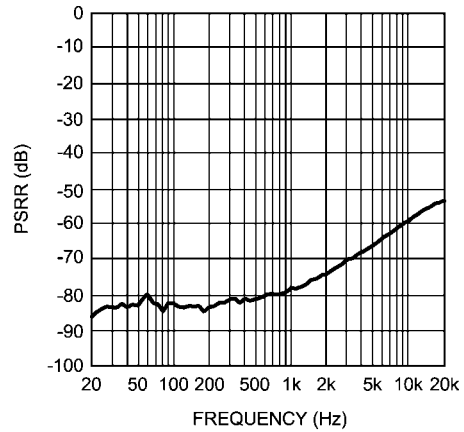
PSRR vs Frequency R_L = 32\Omega , HPV_{DD} = 1.8V , V_{DD} = 5V A_V = 6dB , Mode 4
