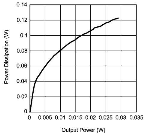
Power Dissipation vs Output Power R_L = 16\Omega , f = 1\text{kHz} , V_{DD} = 1.8\text{V}
