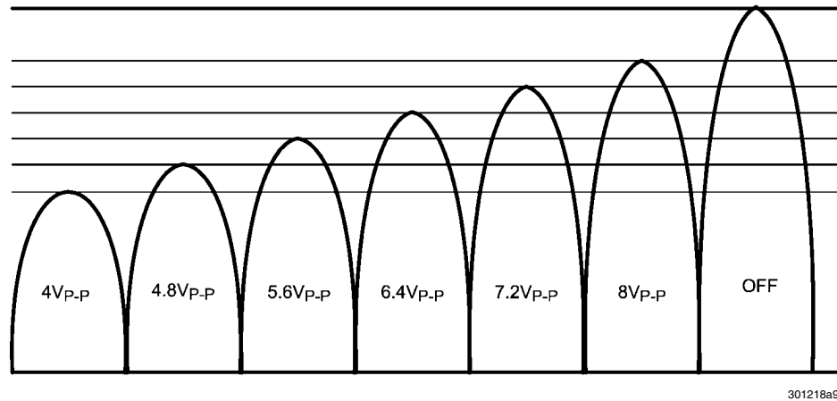
FIGURE 10. Voltage Limit Output Level
