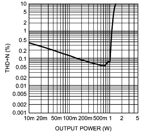
THD+N vs Output Power V_{DD} = 3.6V, R_L = 15\mu H + 4\Omega + 15\mu H f = 1kHz, \text{Mode 2}
