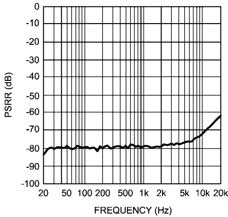
PSRR vs Frequency R_L = 15\mu H + 8\Omega + 15\mu H , V_{DD} = 5V A_V = 6dB , Mode 3
