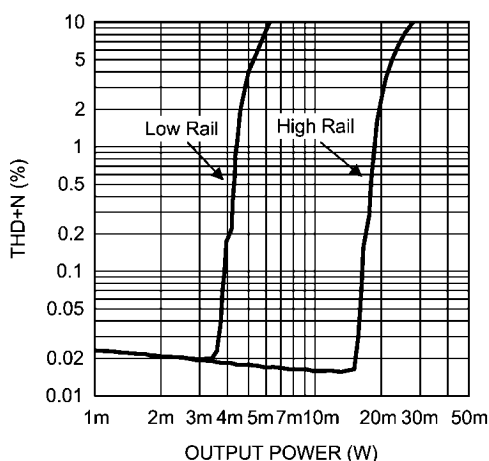
FIGURE 9. Class G Disabled (Low/High Supply Rails)
