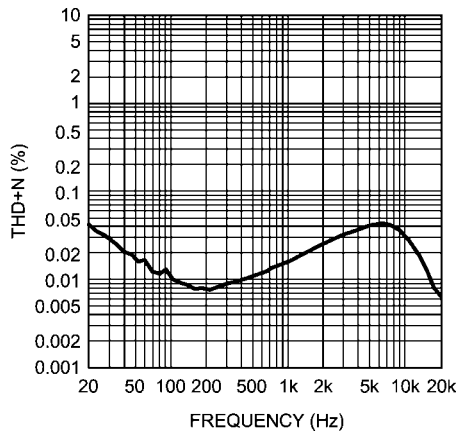
THD+N vs Frequency R_L = 32\Omega P_{OUT} = 14mW, \text{Mode 6}
