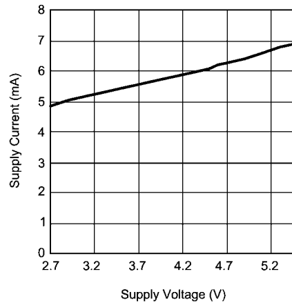
Supply Current vs Supply Voltage Mode 2, Stereo Inputs
