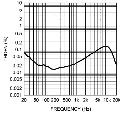
THD+N vs Frequency V_{DD} = 5V, R_L = 5\mu H + 8\Omega + 15\mu H P_{OUT} = 750mW, \text{Mode 2}
