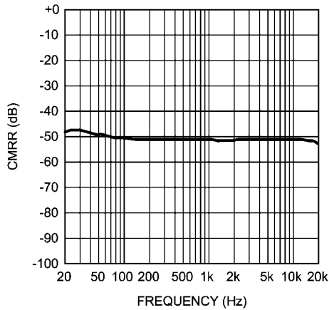
CMRR vs Frequency LS Mode
