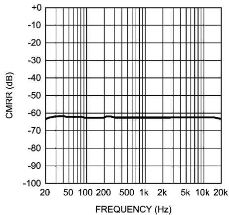
CMRR vs Frequency HP Mode
