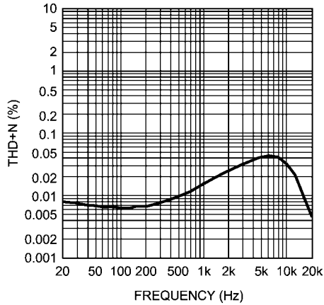
THD+N vs Frequency R_L = 32\Omega P_{OUT} = 14mW, \text{Mode 4}
