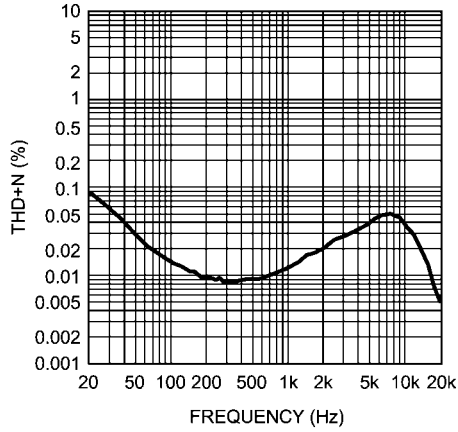
THD+N vs Frequency V_{DD} = 5V, R_L = 15\mu H + 8\Omega + 15\mu H P_{OUT} = 50mW, \text{Mode 3}
