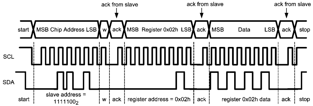
FIGURE 6. Example I 2 C Write Cycle
