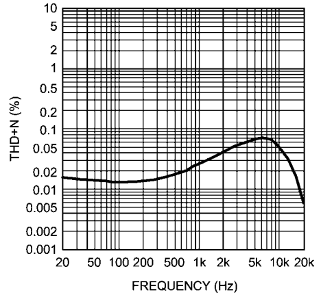
THD+N vs Frequency R_L = 16\Omega P_{OUT} = 14mW, \text{Mode 4}
