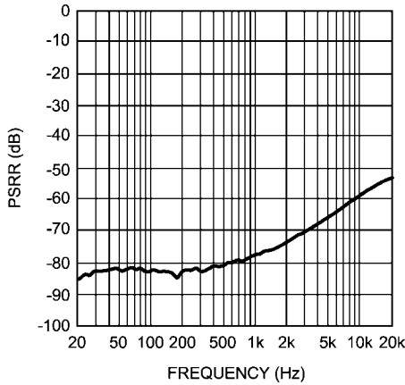
PSRR vs Frequency R_L = 32\Omega , HPV_{DD} = 1.8V , V_{DD} = 5V A_V = 6dB , Mode 6
