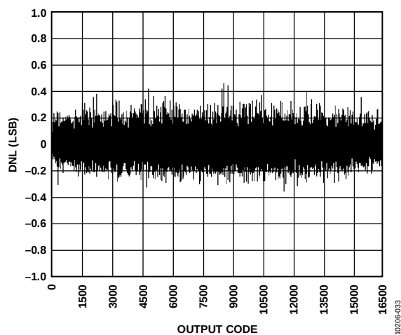
Figure 34. DNL, f_{IN} = 9.7 \text{ MHz} , f_{SAMPLE} = 40 \text{ MSPS}
