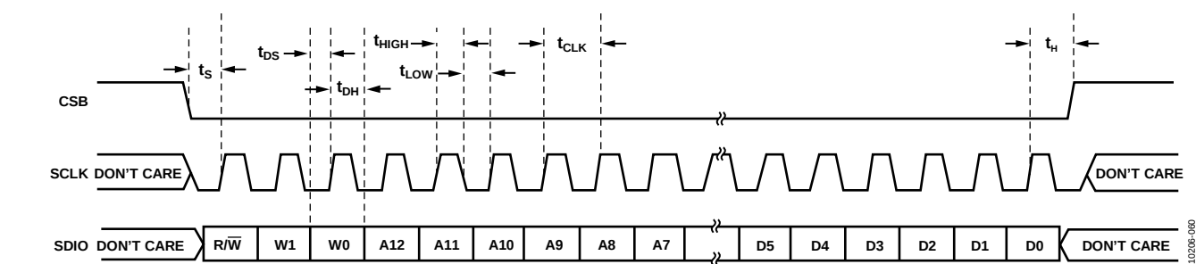
Figure 61. Serial Port Interface Timing Diagram
