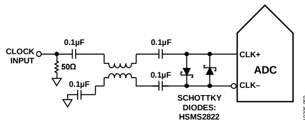
Figure 51. Balun-Coupled Differential Clock (65 MHz to 520 MHz)
