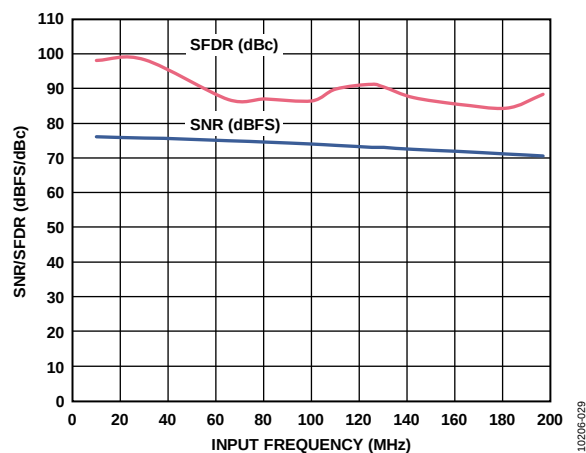
Figure 30. SNR/SFDR vs. f_{IN} , f_{SAMPLE} = 40 MSPS
