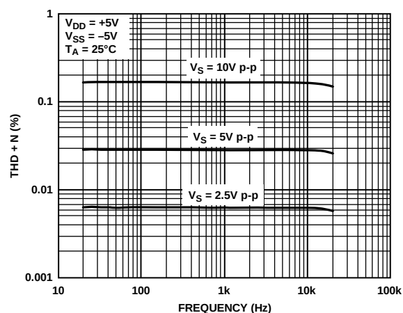
Figure 20. THD + N vs. Frequency at \pm 5 V
