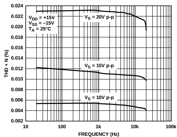
Figure 19. THD + N vs. Frequency at \pm 15 V
