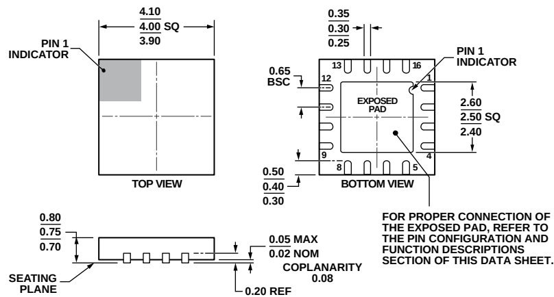
COMPLIANT TO JEDEC STANDARDS MO-220-WGGC. Figure 34. 16-Lead Lead Frame Chip Scale Package [LFCSP] 4 mm × 4 mm Body and 0.75 mm Package Height (CP-16-26)
